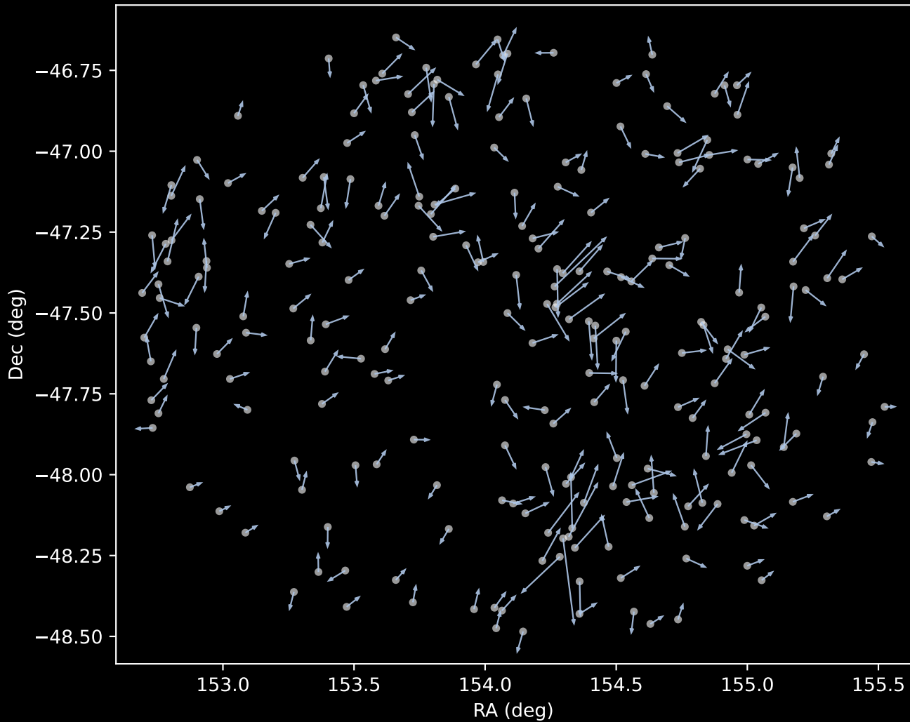
GALAH DR4 Cluster 1 Proper Motion Vectors (n=239)
