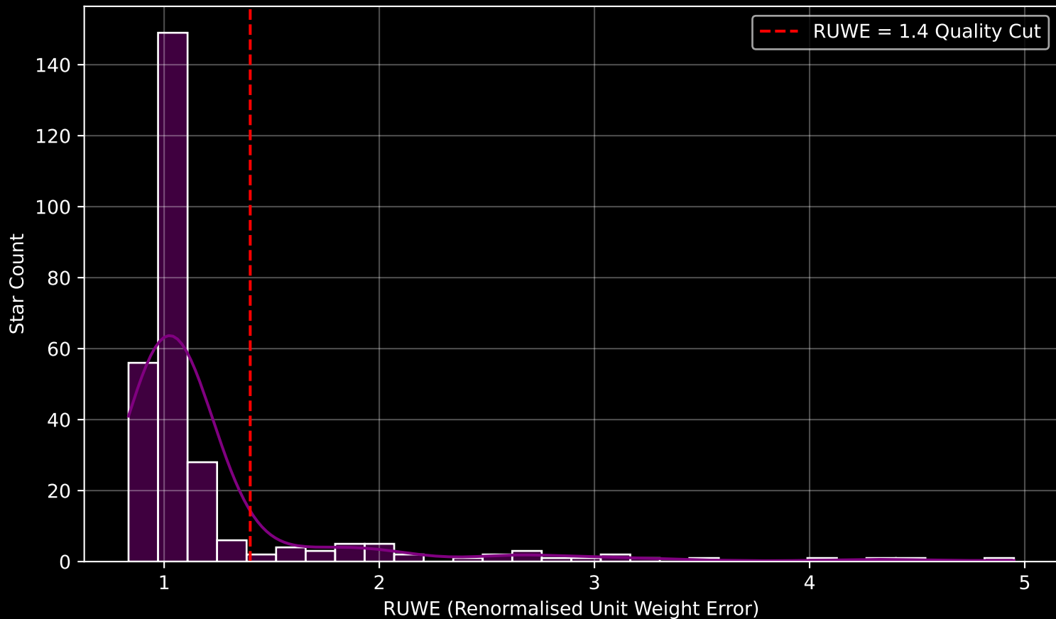
GALAH DR4 Field [6954] RUWE Distribution (n= 276)
