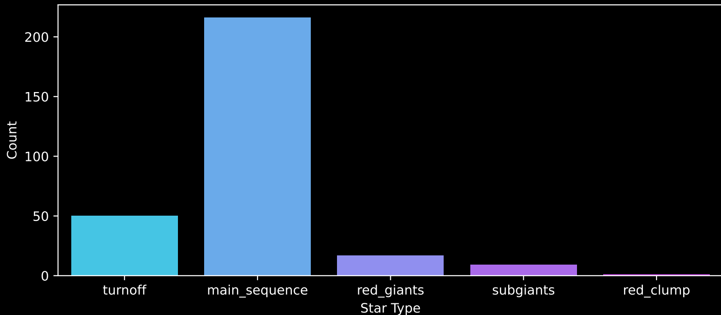
GALAH DR4 Field: [6954] Count plot of Star Type
